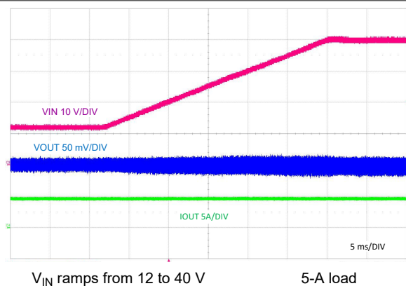
Figure 9-34. Line Transient Response to V_{IN} = 40 V
