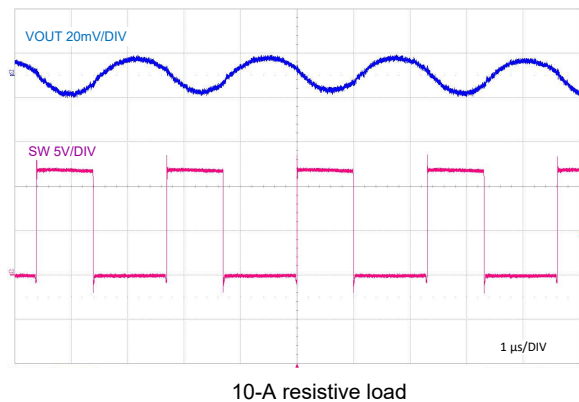
Figure 9-32. Full load Switching
