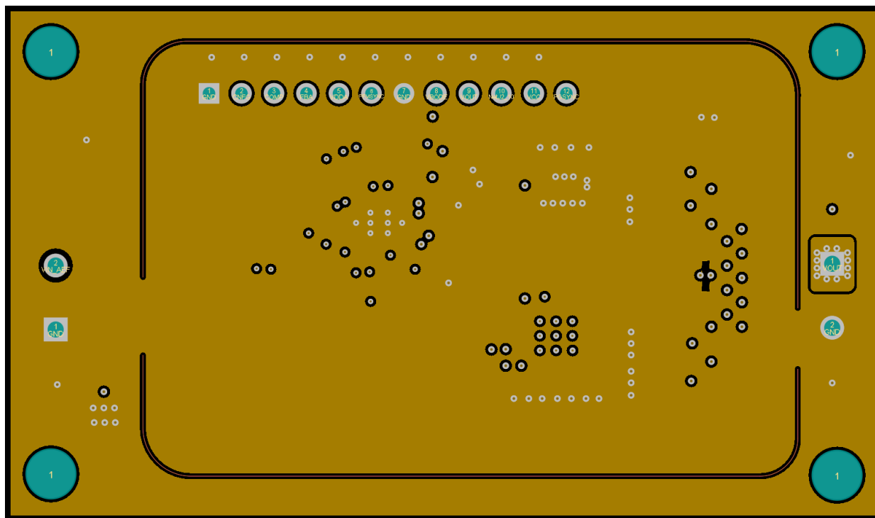
Figure 9-49. Layer 2 Full Ground Plane Directly Under the Power Components
