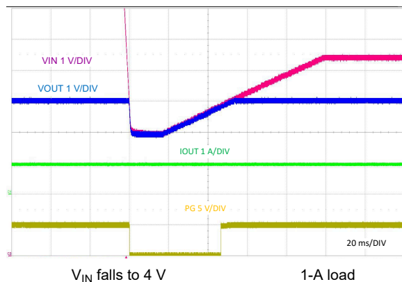
Figure 9-35. Line Transient Response to V_{IN} = 4 V
