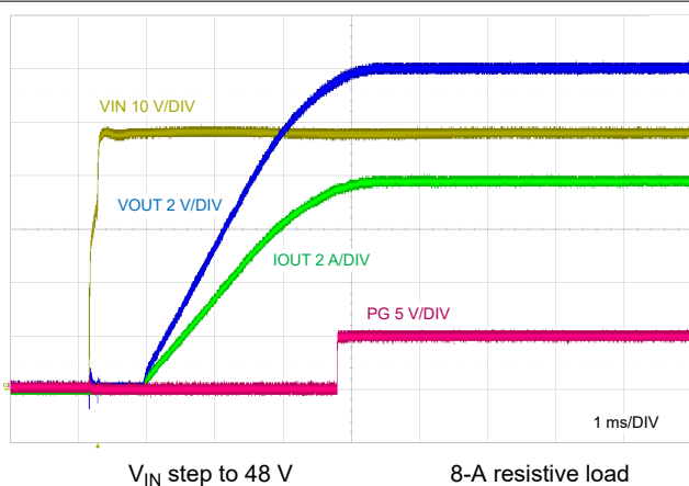
Figure 8-22. Start-Up Characteristic
