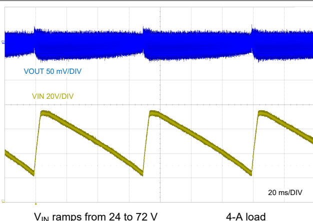
Figure 8-23. Line Transient Response to V_{IN} = 72 V
