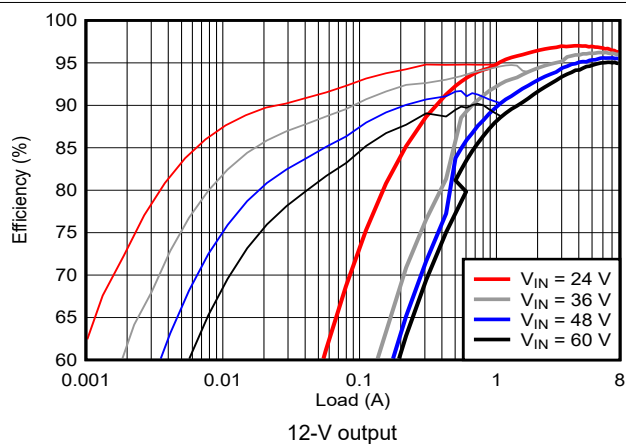
Figure 8-19. Efficiency vs I_{OUT} , Log Scale
