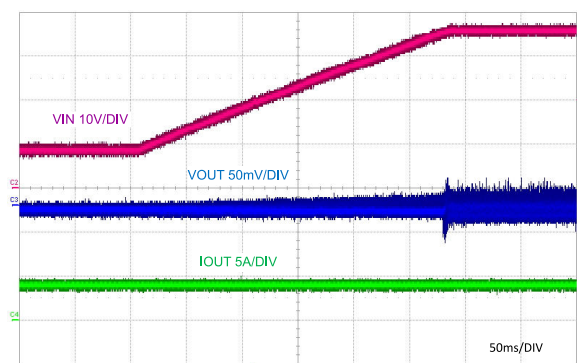
Figure 8-7. Full Load Switching
