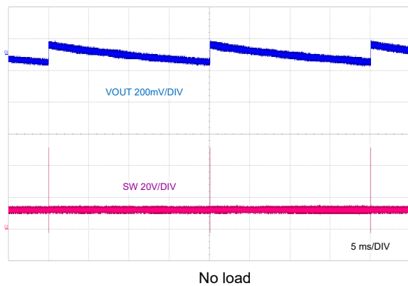
Figure 8-21. PFM Switching
