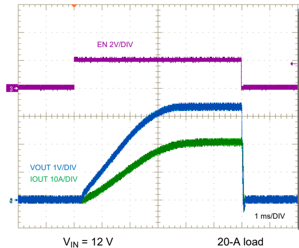
Figure 8-43. ENABLE ON and OFF Characteristic
