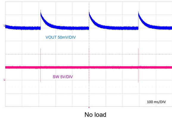
Figure 8-32. PFM Switching
