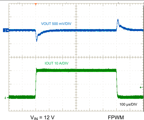
Figure 8-45. Load Transient, 0 A to 20 A
