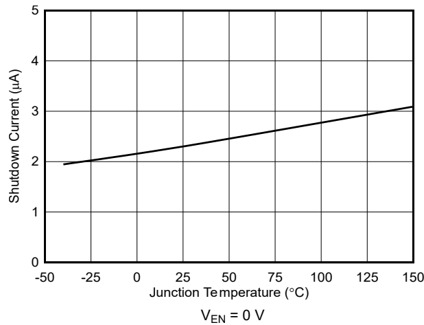
Figure 6-3. Shutdown Current vs Temperature
