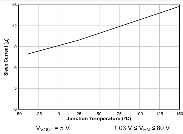
Figure 6-5. Sleep2 Current vs Temperature
