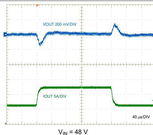
Figure 9-11. Load Transient Response, 6 A to 12 A to 6 A
