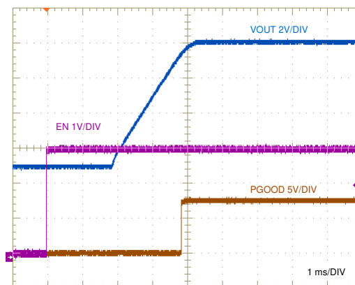
Figure 9-28. Pre-Biased Start-Up
