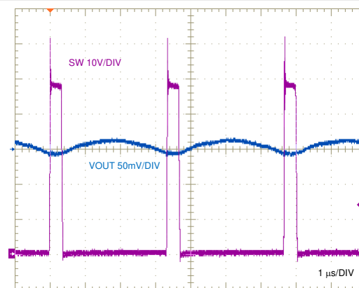
Figure 9-15. SW Node and Output Ripple Voltages
