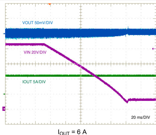
Figure 9-14. Line Transient Response, 85 V to 12 V
