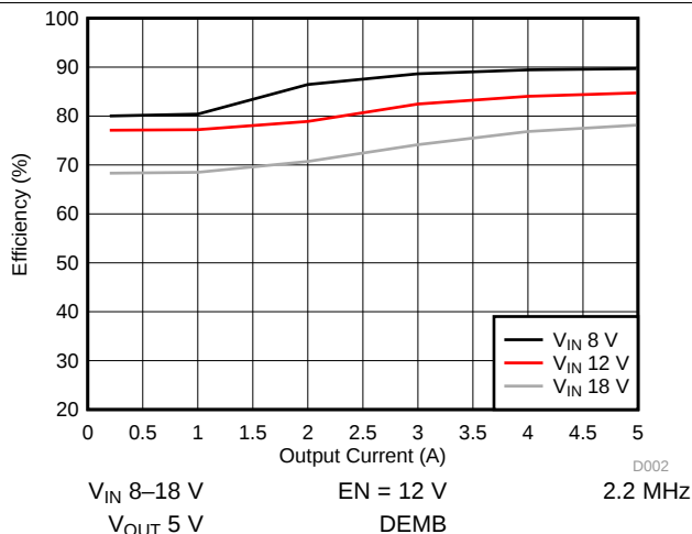
Figure 2. Efficiency vs I_{OUT}
