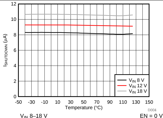
Figure 4. I_{SHUTDOWN} vs Temperature
