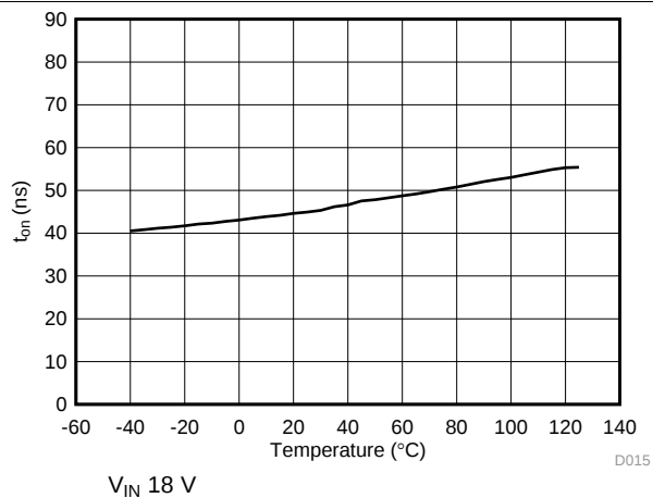
Figure 15. t_{\text{on}} Minimum vs Temperature
