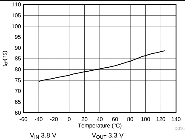
Figure 16. t_{\text{off}} Minimum vs Temperature
