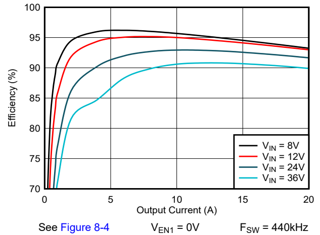
Figure 6-2. Efficiency vs Load, 3.3V Output
