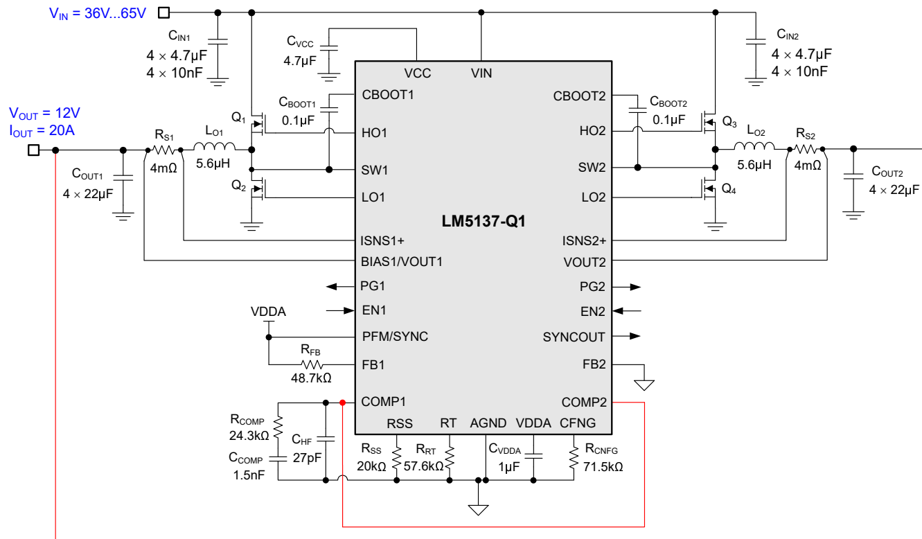
Figure 8-20. Application Circuit 3 With an LM5137-Q1 Two-phase Buck Regulator at 400kHz
