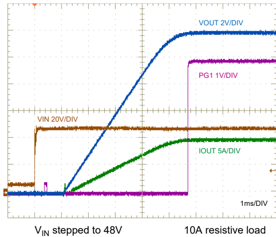
Figure 8-23. Start-Up Characteristic
