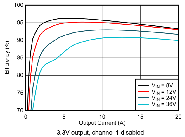
Figure 8-6. Efficiency vs I_{OUT2}
