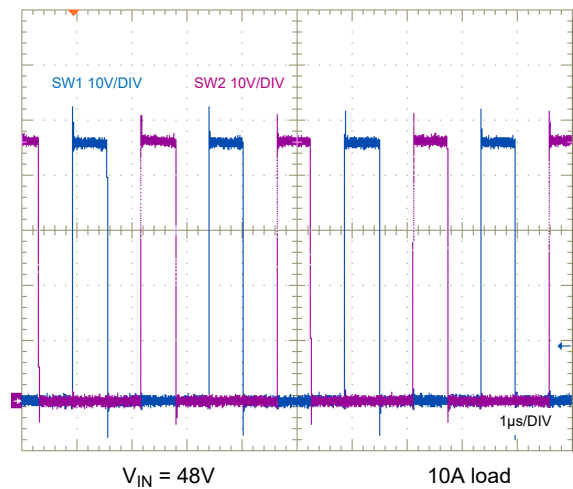
Figure 8-26. Switch-node Voltages
