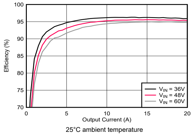
Figure 8-21. Efficiency vs I_{OUT} , PFM/SYNC Tied Low
