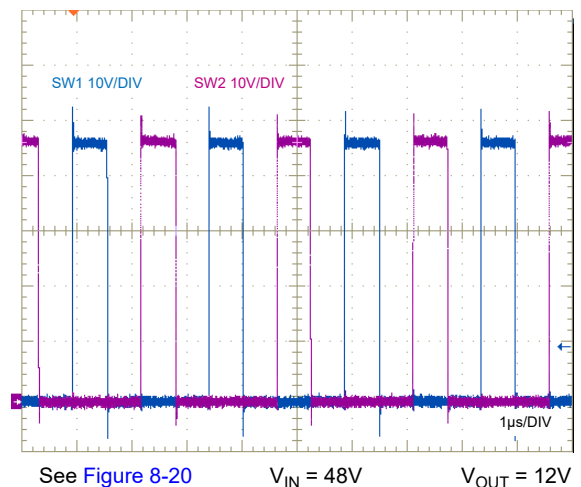
Figure 6-6. Switch-Node Voltages
