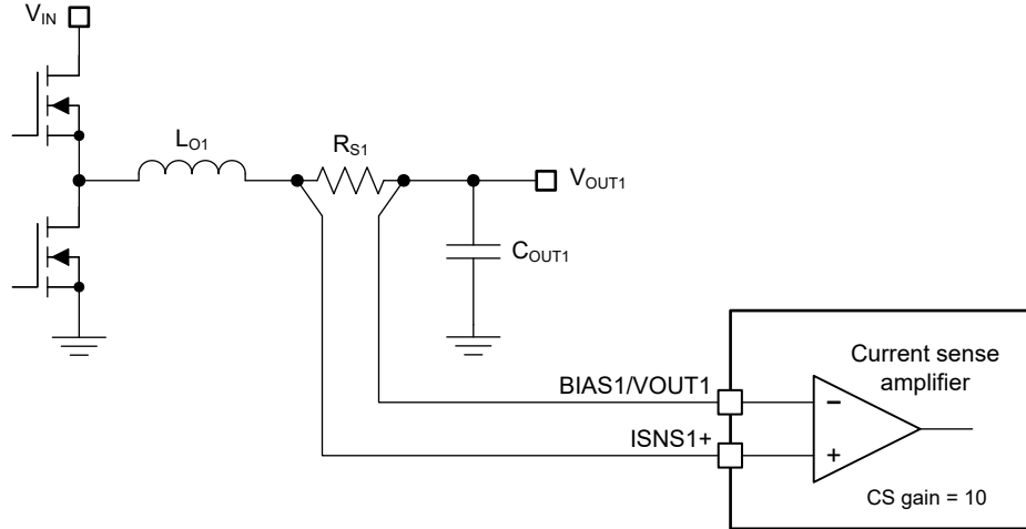
Figure 7-5. Shunt Current Sensing Implementation
