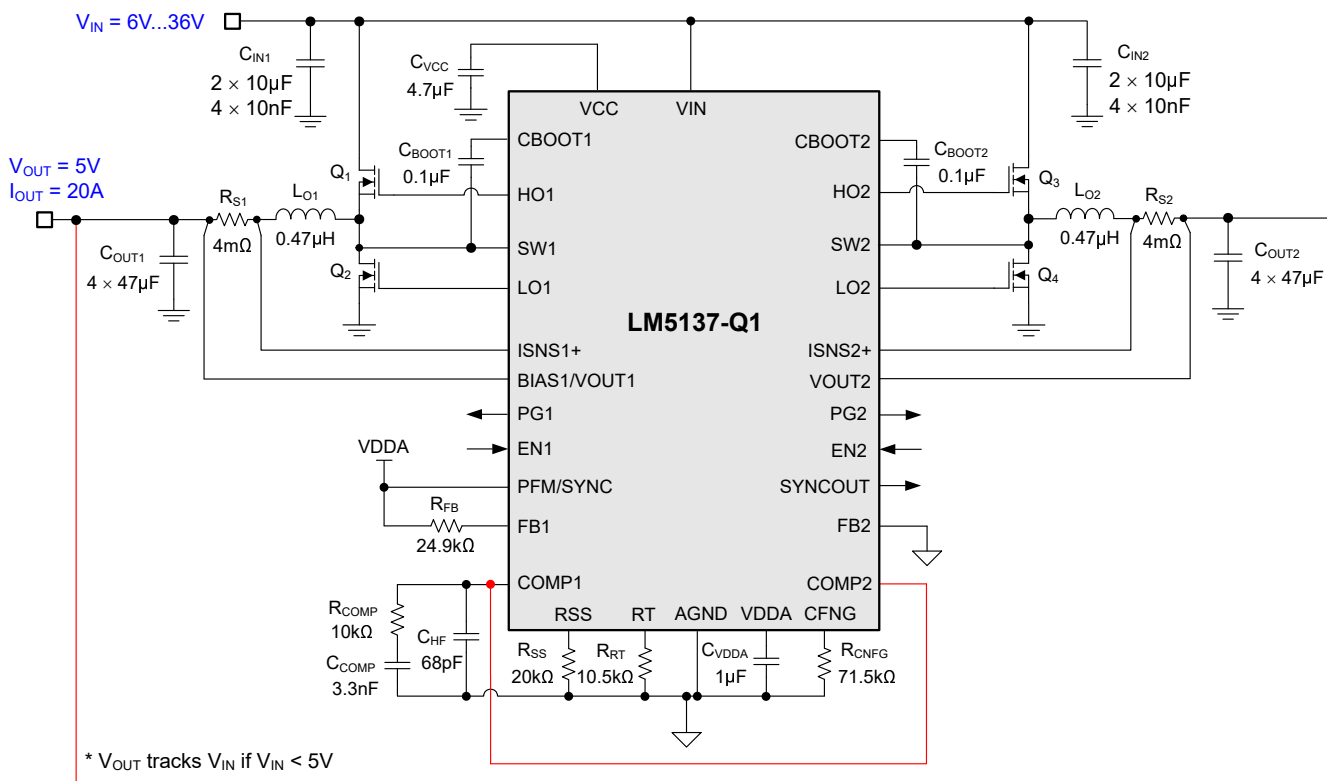
Figure 8-19. Application Circuit 2 With an LM5137-Q1 Two-phase Buck Regulator at 2.1MHz
