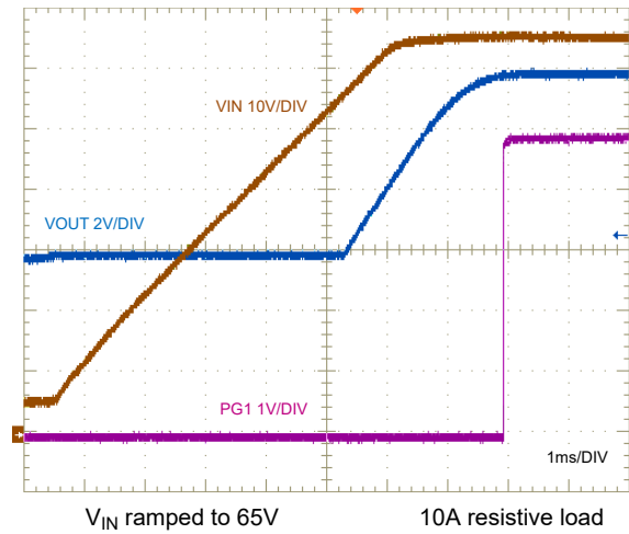
Figure 8-24. Prebiased Start-Up Characteristic
