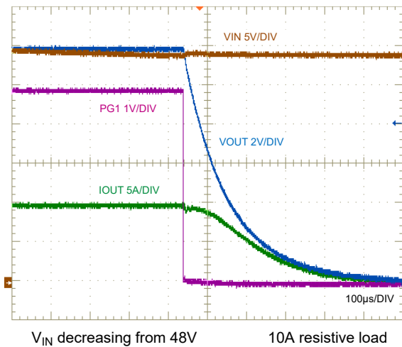
Figure 8-25. Shutdown Characteristic
