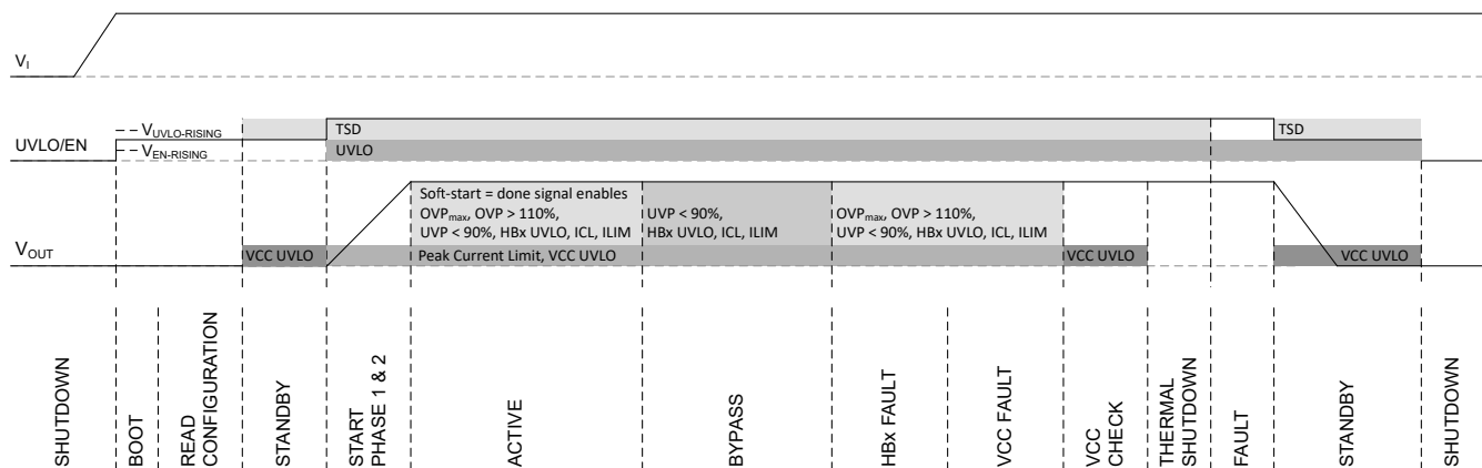
Figure 6-18. Protections
