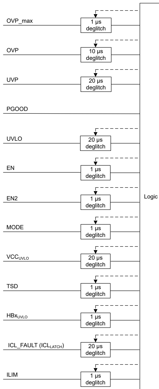
Figure 6-17. Signal Deglitching
