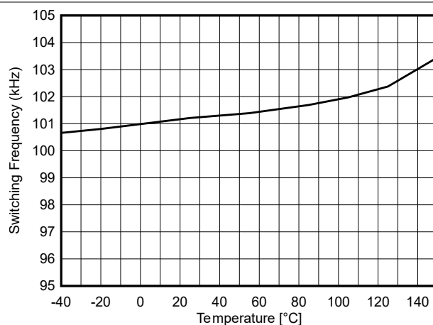
Figure 5-2. Switching Frequency (100kHz, RT = 316kΩ) vs Temperature
