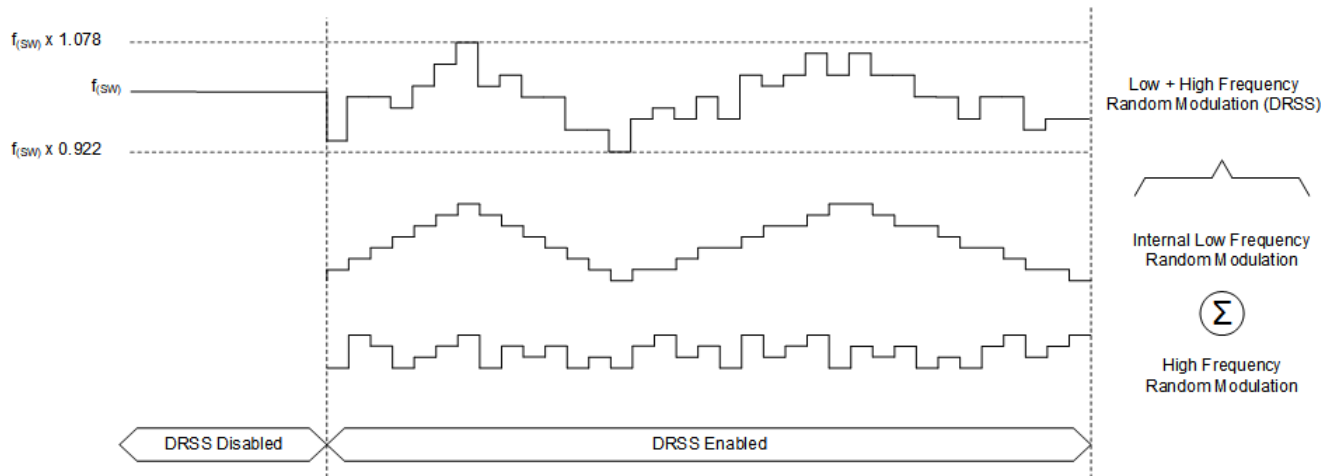
Figure 6-4. Dual Random Spread Spectrum
