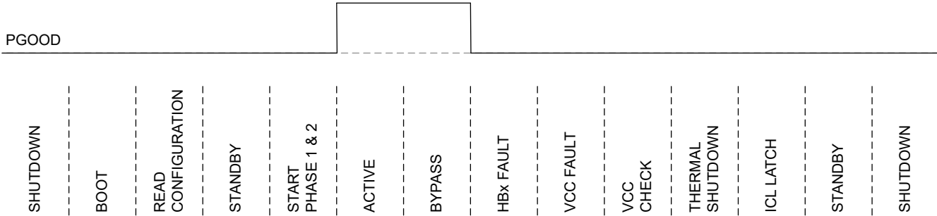
Figure 6-12. PGOOD Status for All Device States
