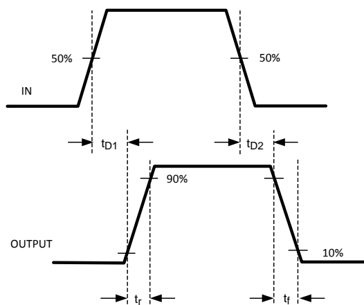
Figure 13. Non-Inverting
