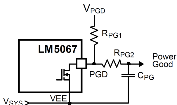
Figure 9-14. Adding Delay to the Power Good Output Pin - Long Delay at Rising Edge, Short Delay at Falling Edge
