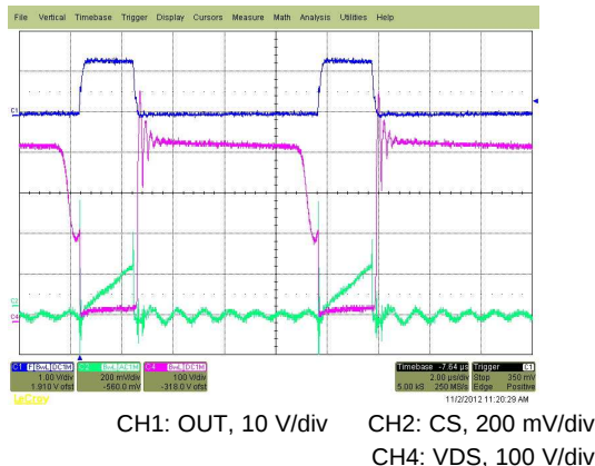
Figure 24. QR Waveforms V_{IN} 230 V AC , I_{OUT} 3.43 A
