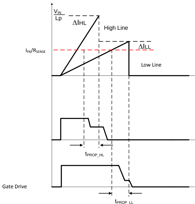
Figure 15. Line-Current Feedforward
