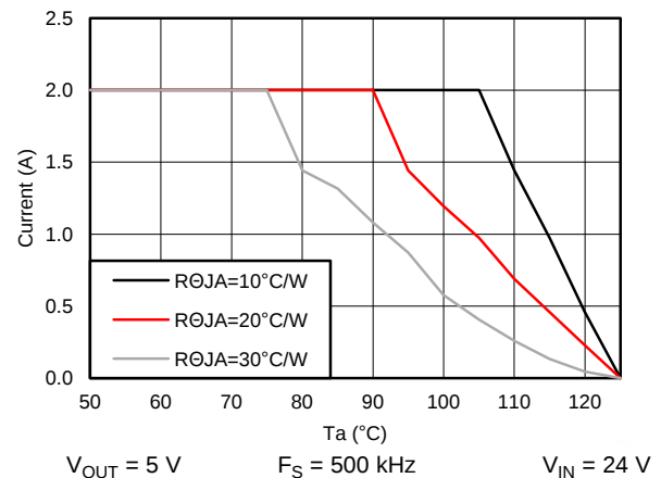
Figure 58. Derating Curve
