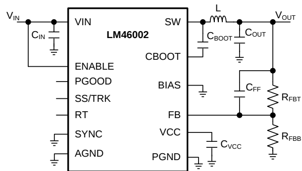
Figure 45. LM46002 Basic Schematic for V_{OUT} < 3.3\text{ V} , t-Tie BIAS to Ground
