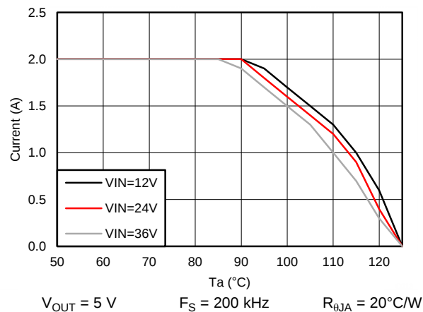
Figure 85. Derating Curve with R_{\theta JA} = 20^\circ\text{C/W}
