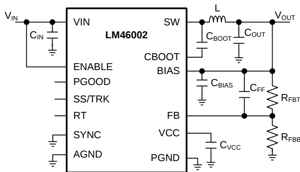
Figure 44. LM46002 Basic Schematic for V_{OUT} \geq 3.3\text{ V} , Tie BIAS to V_{OUT}
