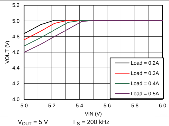
Figure 62. Dropout Curve
