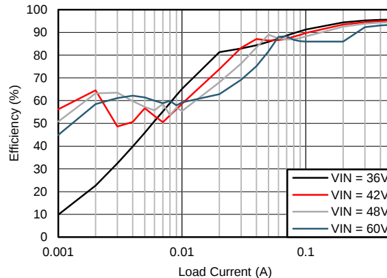
Figure 78. Efficiency
