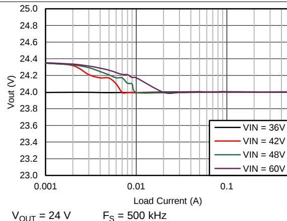
Figure 12. V_{OUT} Regulation
