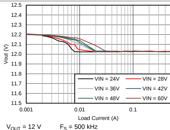
Figure 11. V_{OUT} Regulation
