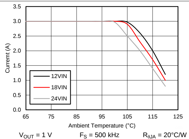
Figure 54. Derating Curve
