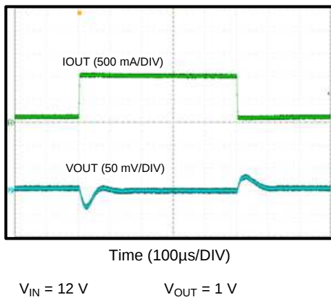
Figure 53. Load Transient 0.1A to 1A
