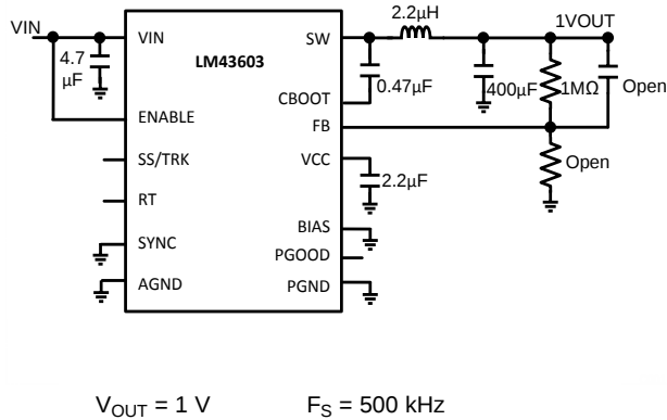
Figure 49. BOM for V_{OUT}= 1\text{V} F_S = 500\text{kHz}
