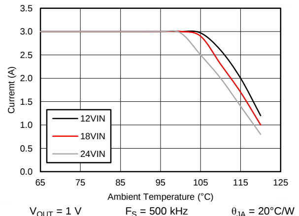
Figure 54. Derating Curve
