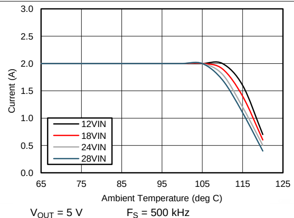
Figure 62. Derating Curve
