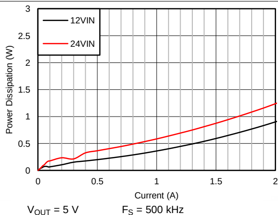
Figure 55. Power Dissipation at Room Temperature
