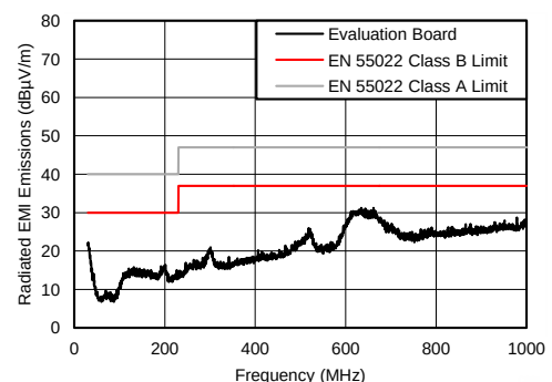
Radiated Emission Graph 12V_{\text{IN}} to 3.3V_{\text{OUT}} F_s = 500\text{ kHz} I_{\text{OUT}} = 2\text{ A}
