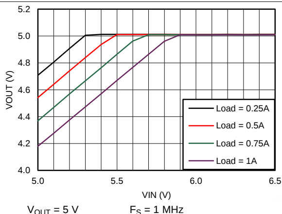
Figure 74. Dropout Curve
