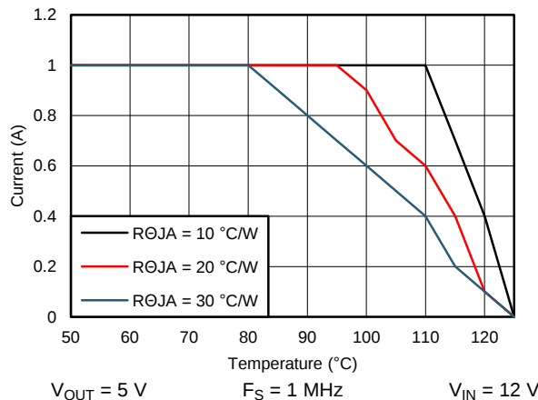
Figure 76. Derating Curve
