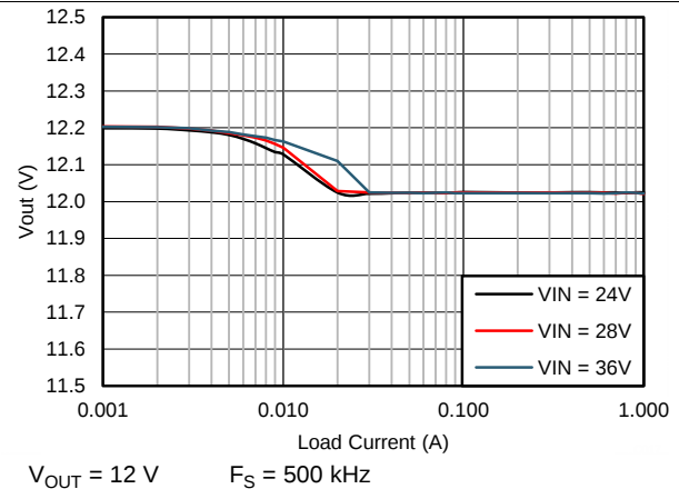
Figure 12. V_{OUT} Regulation
