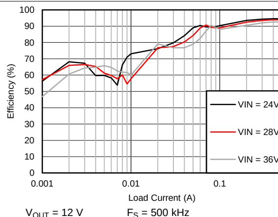
Figure 84. Efficiency
