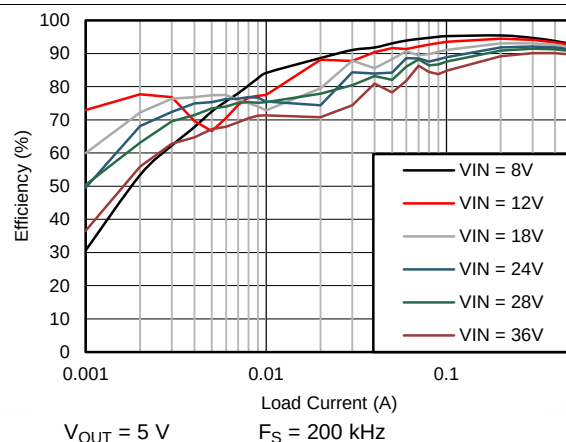
Figure 66. Efficiency
