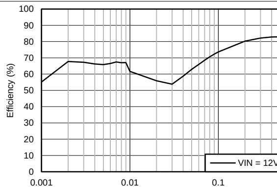
Figure 78. Efficiency
