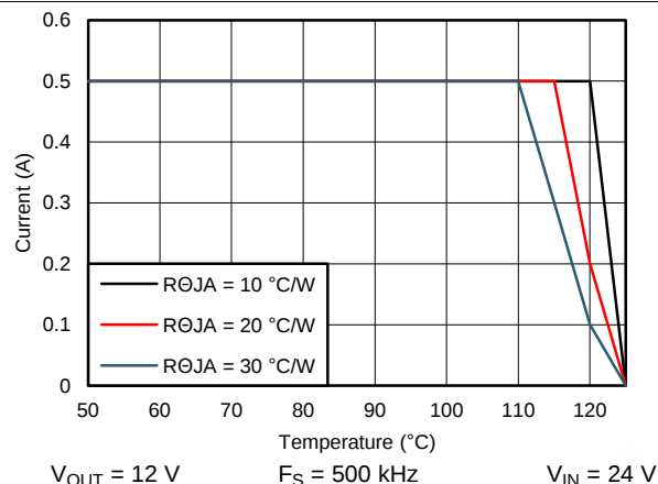
Figure 88. Derating Curve
