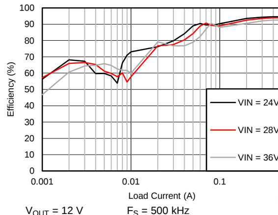
Figure 84. Efficiency
