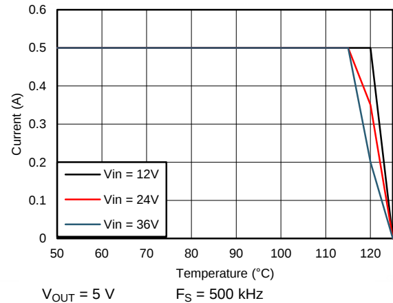
Figure 90. Derating Curve with R_{\theta JA} = 20^\circ\text{C/W}
