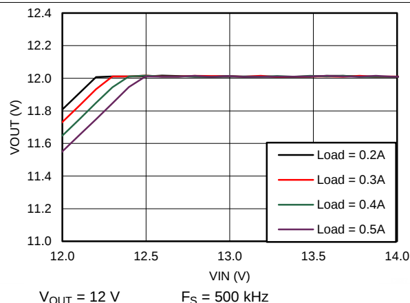
Figure 86. Dropout Curve
