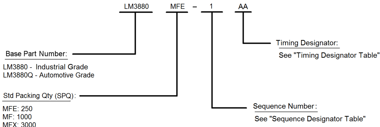
Figure 10-1. Device Nomenclature
