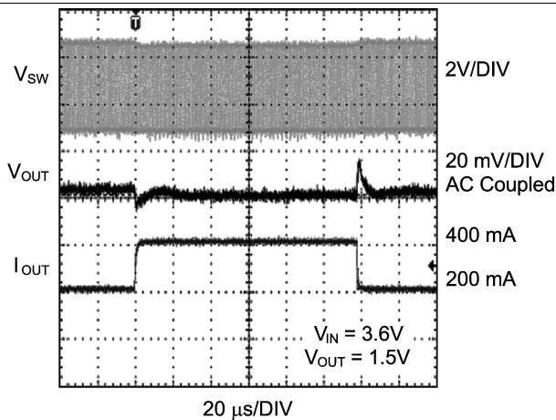
Figure 15. Load Transient
