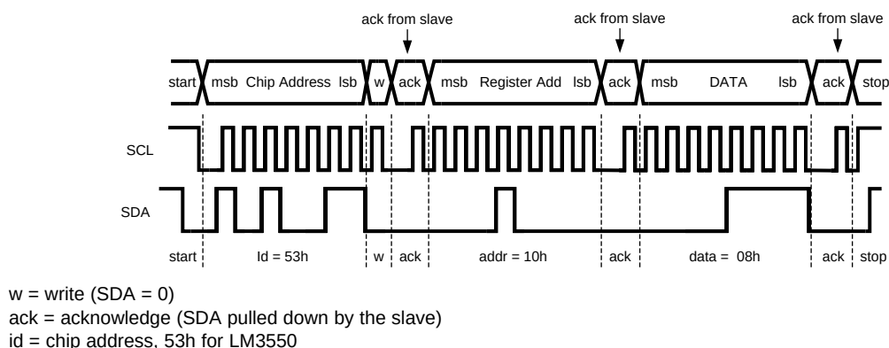
Figure 46. Write Cycle
