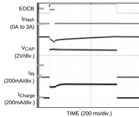
Figure 61. 5.3-V Mode Super Capacitor Charge
