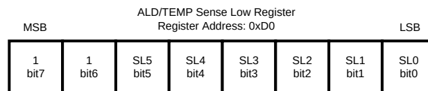
Figure 48. ALD/TEMP Sense Low Register
