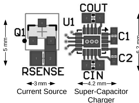
Figure 72. LM3550 Layout
