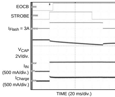
Figure 63. 5.3-V Mode Super Capacitor Recharge
