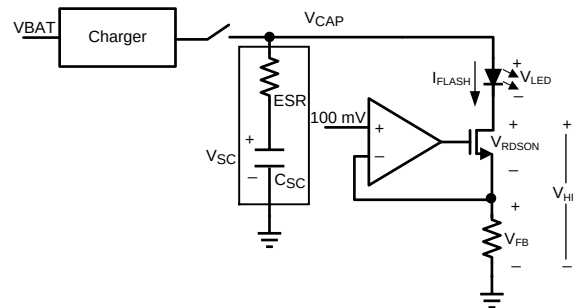
Figure 37. Power Loss Model
