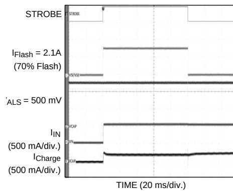
Figure 33. Flash With \overline{\text{FGATE}} = 1
