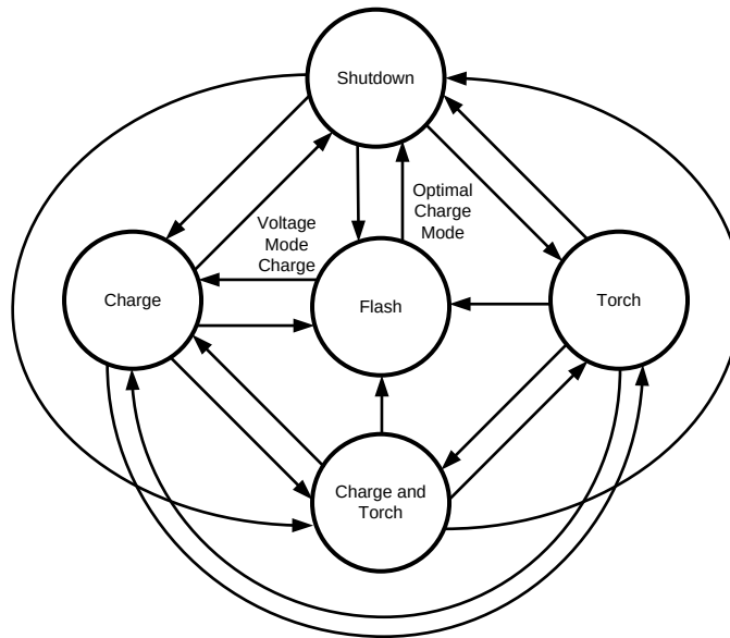
Figure 41. \overline{\text{FGATE}} = 1 State Diagram
