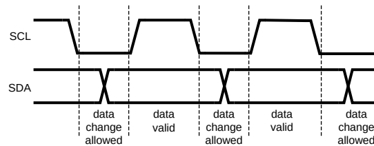
Figure 44. Data Validity Diagram
