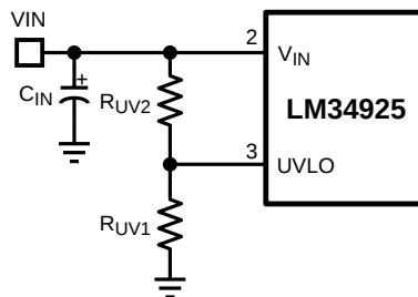
Figure 10. UVLO Resistor Setting
