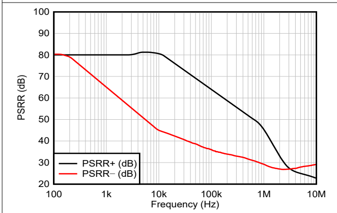
Figure 5-9. PSRR vs Frequency
