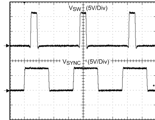
Figure 16. Frequency Synchronization
