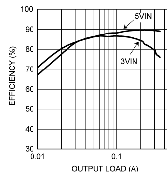
Efficiency vs Load Current V_O = 12\text{ V}
