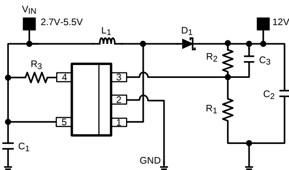
Typical Boost Application Circuit
