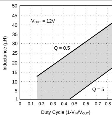
Figure 17. Minimum Inductance Requirements for (a) f_s = 600 kHz
