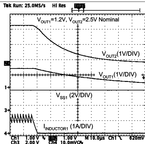
Figure 20. Thermal Shutdown
