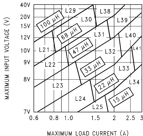
Figure 9-6. LM2596-5.0
