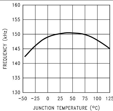
Figure 7-12. Switching Frequency
