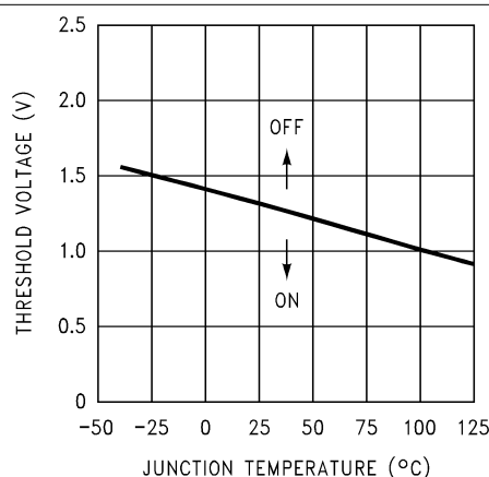
Figure 7-10. \overline{ON/OFF} Threshold Voltage
