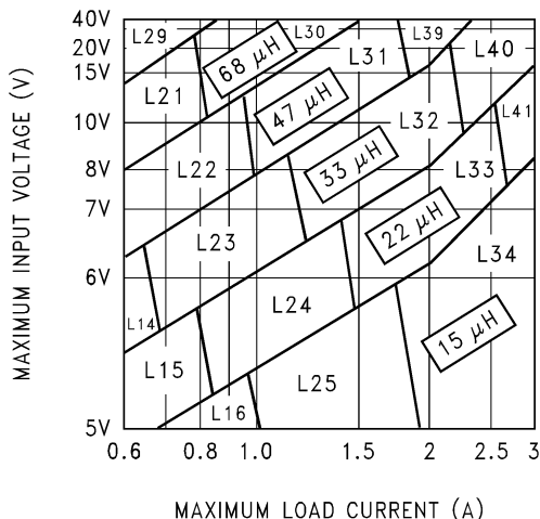
Figure 9-5. LM2596-3.3
