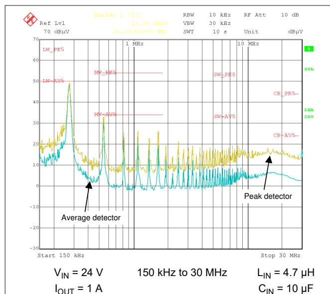
Figure 8-14. CISPR 25 Class 5 Conducted EMI Plot
