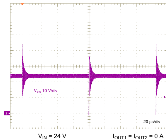
Figure 8-22. Switch Voltage, No Load
