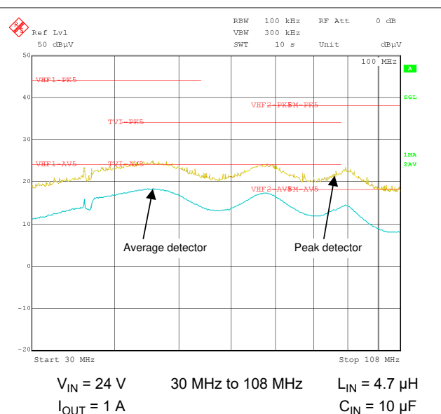
Figure 8-15. CISPR 25 Class 5 Conducted EMI Plot
