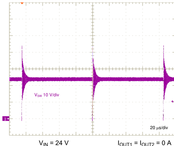
Figure 8-22. Switch Voltage, No Load
