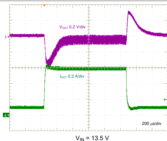
Figure 8-12. Load Transient, 0.1 A to 0.6 A, 0.1 A/ \mu s
