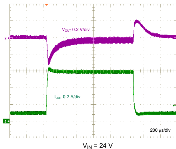
Figure 8-11. Load Transient, 0.1 A to 0.6 A, 0.1 A/ \mu s
