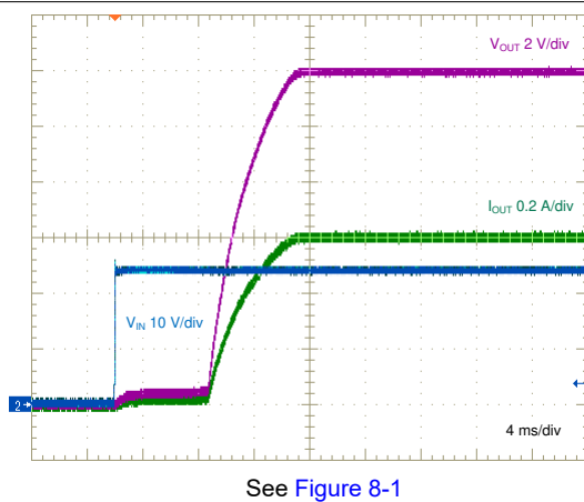
Figure 6-5. Start-up Characteristic
