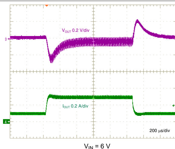
Figure 8-13. Load Transient, 0.1 A to 0.3 A, 0.1 A/ \mu s
