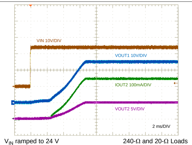
Figure 47. Start-Up Characteristic
