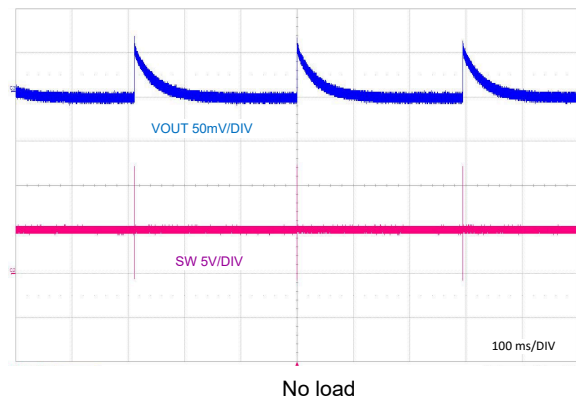
Figure 9-21. PFM Switching
