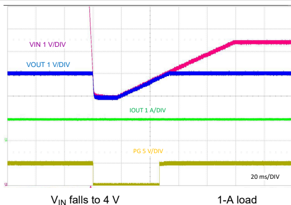
Figure 9-23. Line Transient Response to V_{IN} = 4\text{ V}
