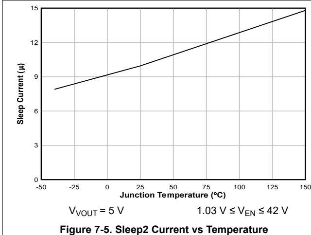
Figure 7-5. Sleep2 Current vs Temperature
