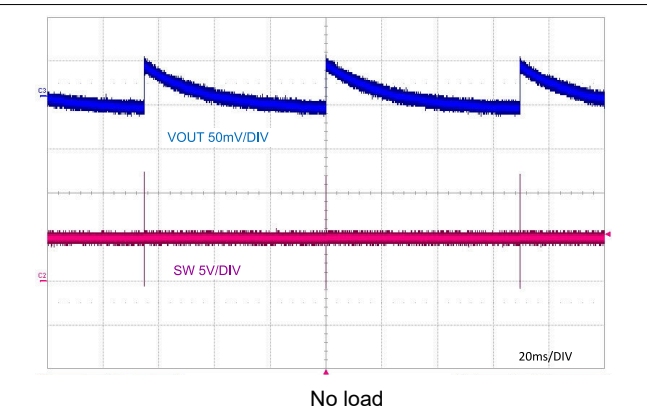
Figure 9-8. PFM Switching
