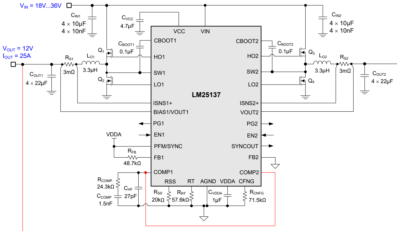
Figure 8-20. Application Circuit 3 With an LM25137 Two-phase Buck Regulator at 400kHz
