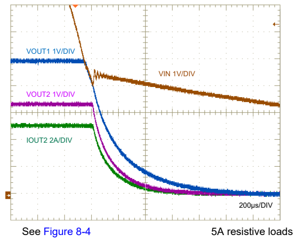
Figure 6-4. Shutdown Characteristic
