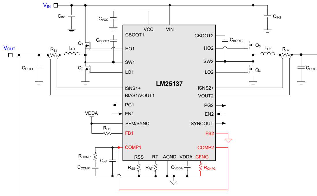
Figure 7-8. LM25137 Two-phase Regulator Schematic Configured for Single-output Interleaved Operation
