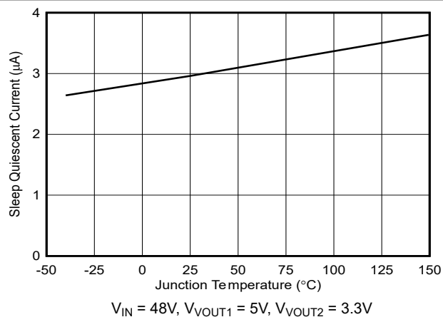
Figure 6-10. Sleep Quiescent Current vs Temperature
