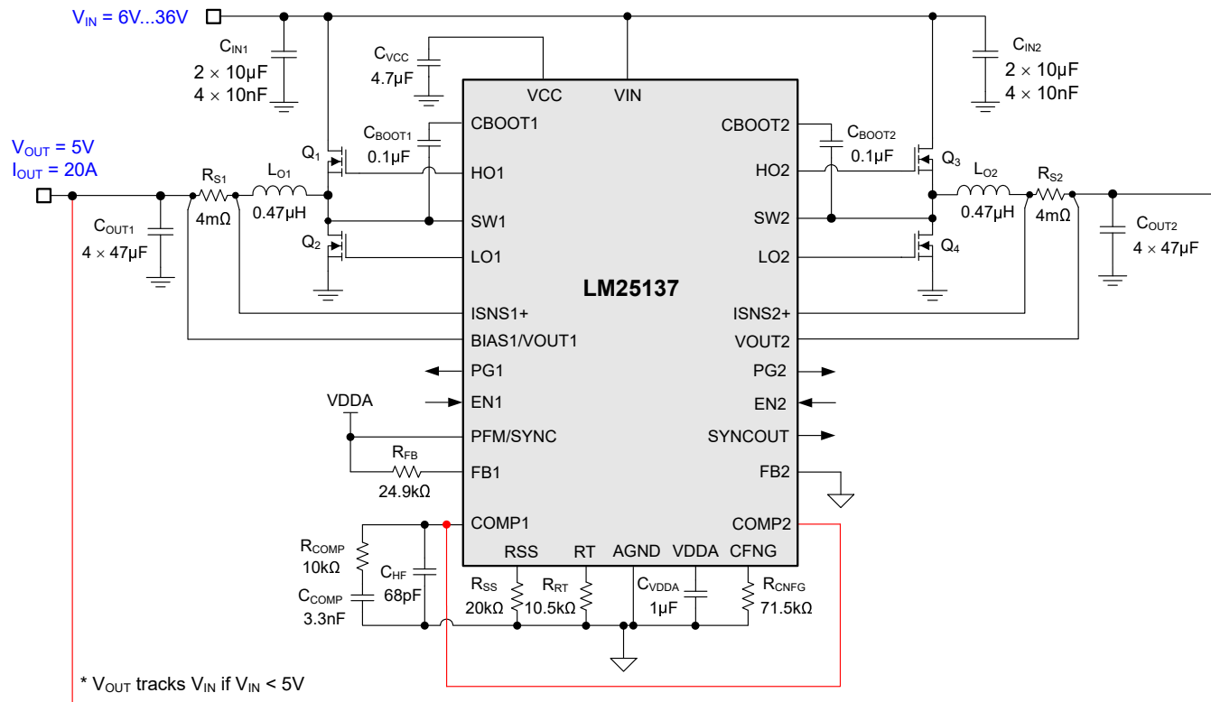
Figure 8-19. Application Circuit 2 With an LM25137 Two-phase Buck Regulator at 2.1MHz
