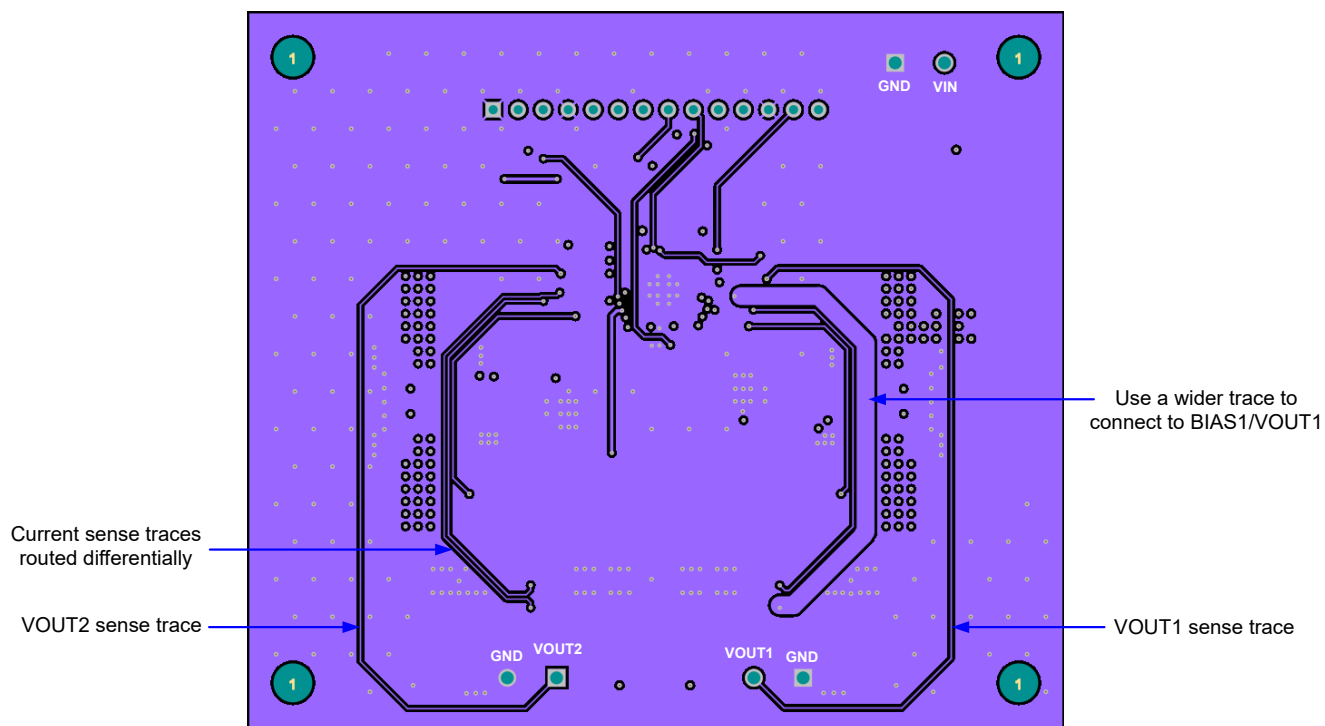
Figure 8-29. PCB Inner Layer
