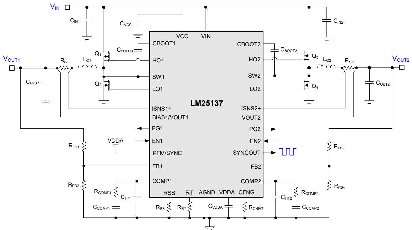
Figure 7-1. LM25137 Dual-Output Regulator Schematic
