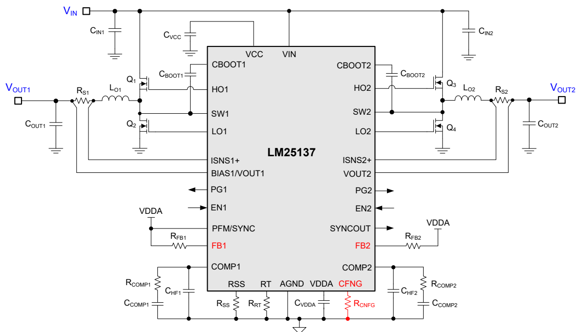
Figure 7-7. LM25137 Regulator Schematic Configured for Independent Dual Outputs
