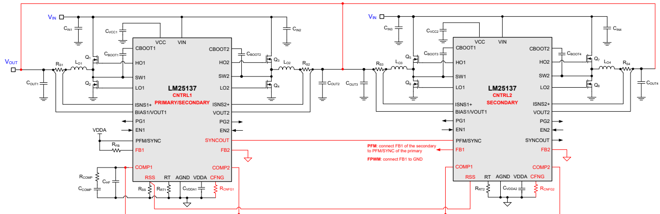
Figure 7-9. LM25137 Multiphase Regulator Schematic Configured for Single-Output Interleaved Operation
