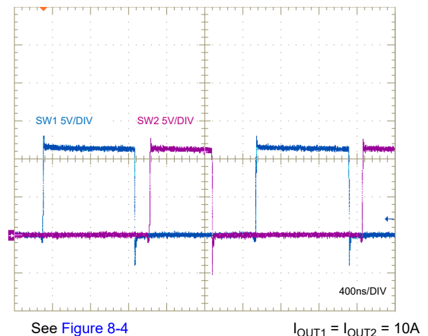
Figure 6-6. Switch-Node Voltages
