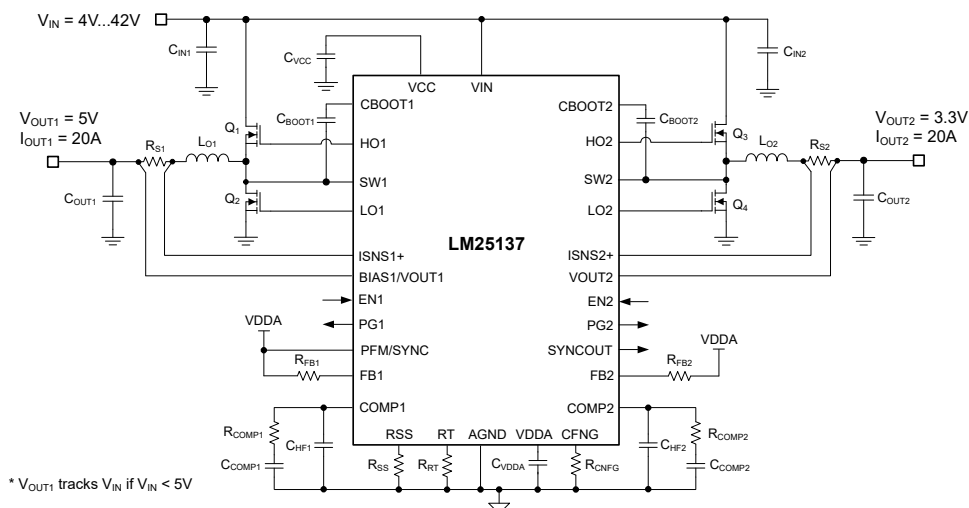
LM25137 Dual-Output Buck Switching Regulator – Simplified Schematic
