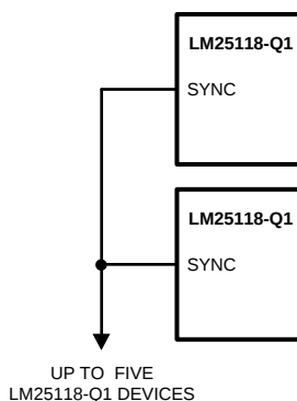
Figure 11. Sync From Multiple Devices
