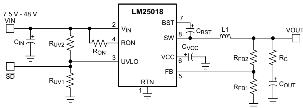
Typical Application
