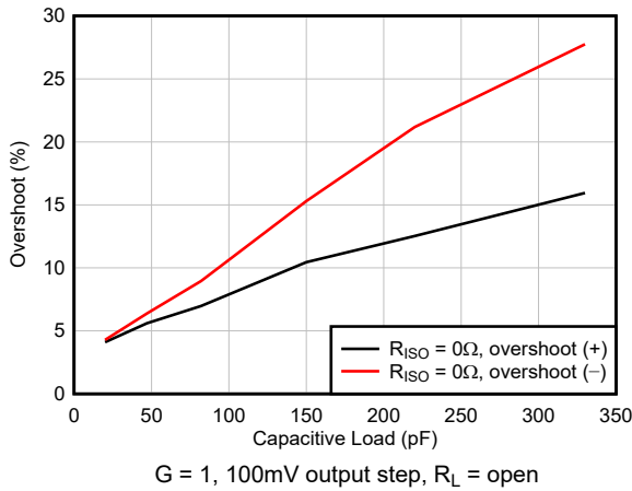
Figure 6-21. Small-Signal Overshoot vs Capacitive Load
