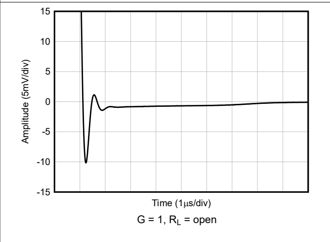
Figure 6-28. Large-Signal Step Response (Falling)
