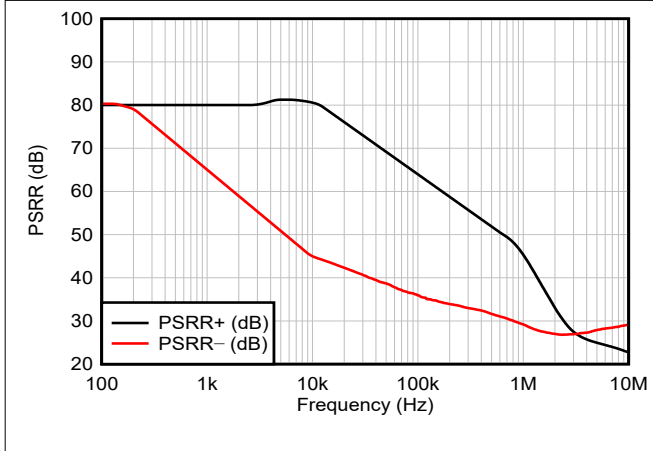
Figure 6-9. PSRR vs Frequency
