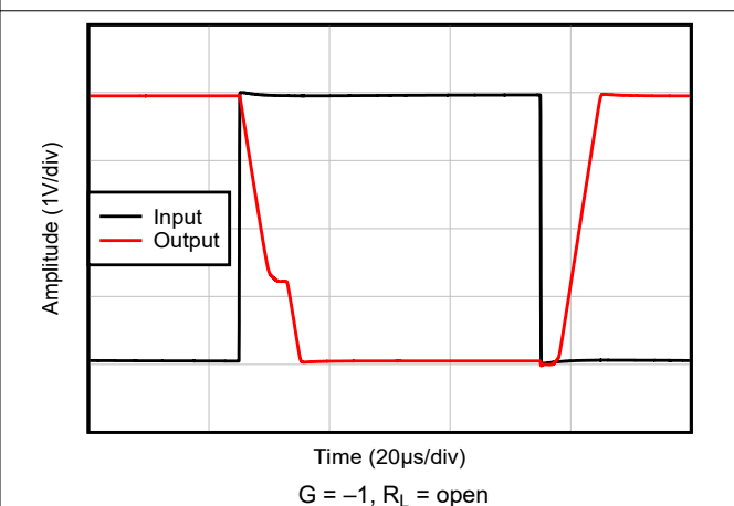
Figure 6-30. Large-Signal Step Response, G = -1
