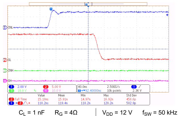
Figure 8-2. GL Fall Time and \overline{\text{INL}} to GL Turn-off Propagation Delay
