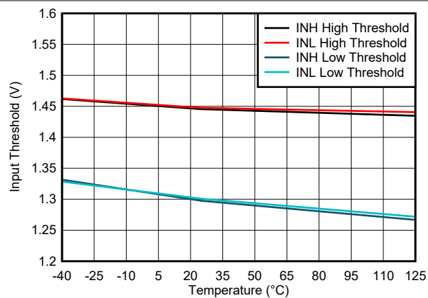
Figure 6-13. Input Voltage Thresholds vs Temperature
