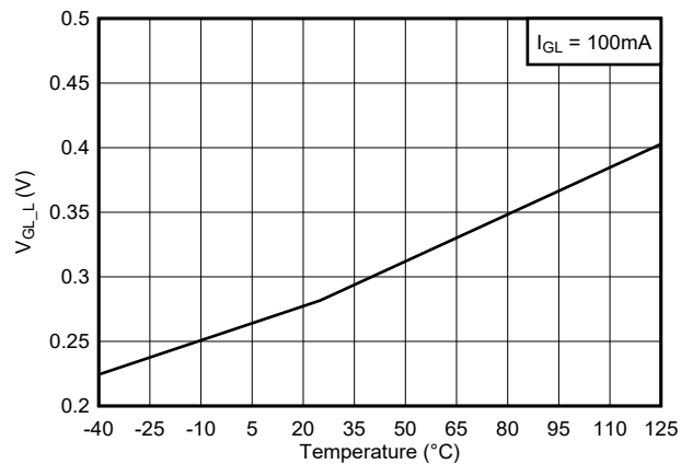
Figure 6-9. GL Output Low Voltage vs Temperature
