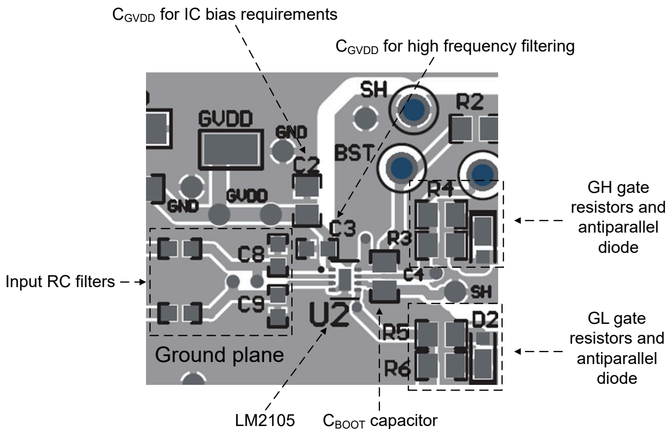
Figure 10-1. Layout Example
