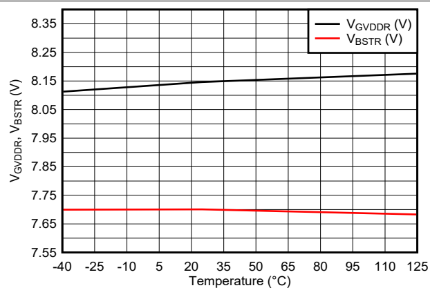
Figure 6-11. GVDD and BST UVLO Thresholds vs Temperature
