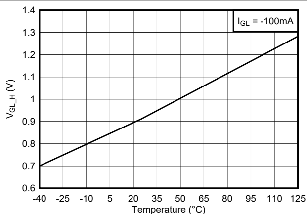
Figure 6-7. GL Output High Voltage vs Temperature
