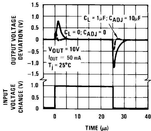
Figure 7-11. Line Transient Response
