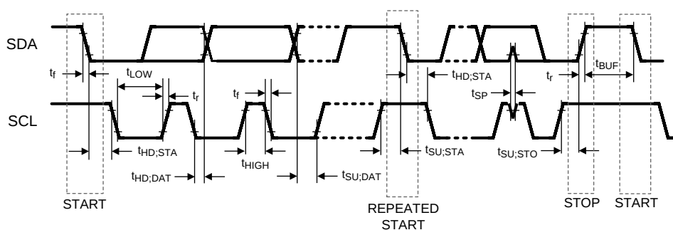
Figure 1. I2C Timing
