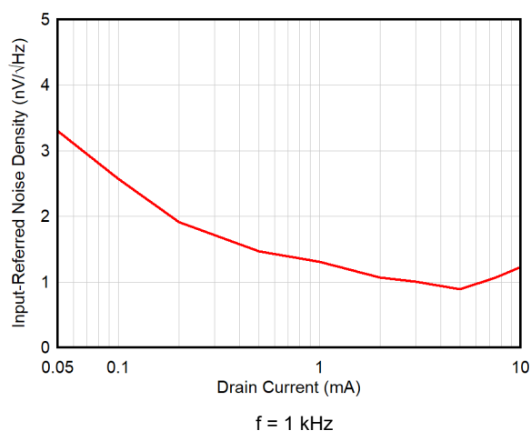
Figure 6-16. Input-Referred Noise Spectral Density vs Drain-to-Source Current
