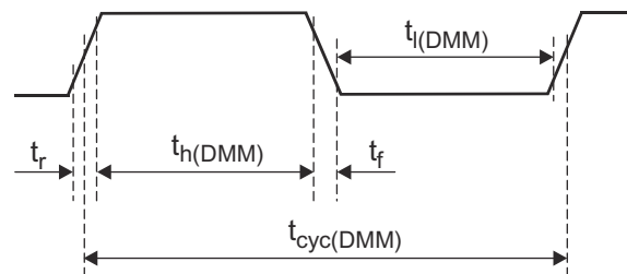
Figure 7-19. DMMCLK Timing
