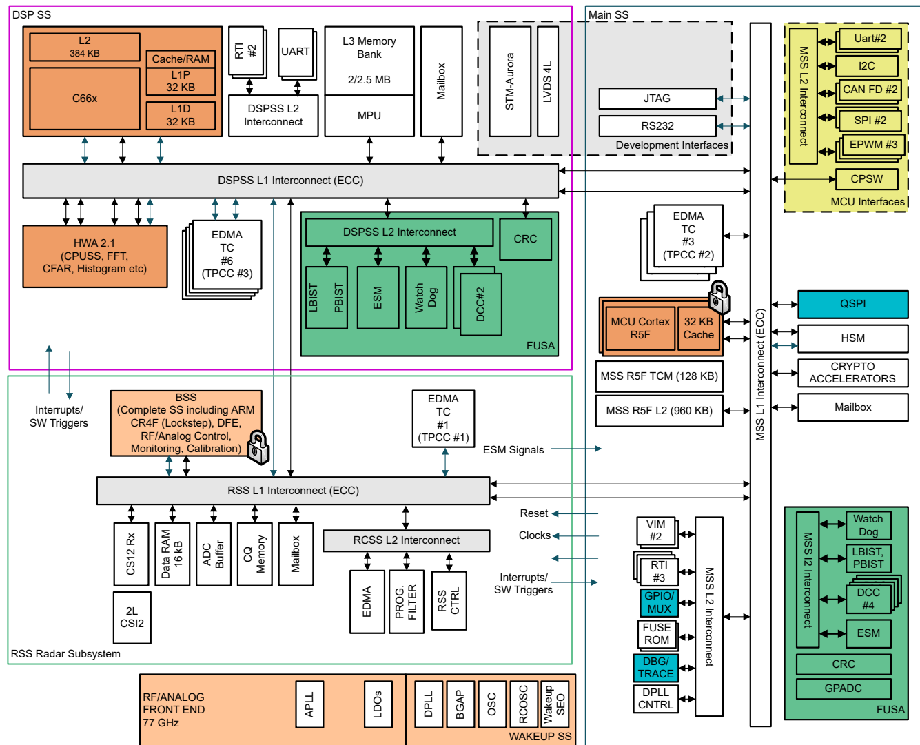
Figure 7-5. Processor subsystem
