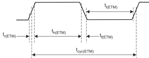
Figure 7-20. ETMTRACECLKOUT Timing
