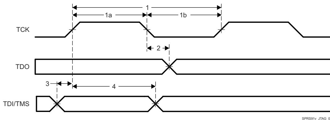
Figure 7-24. JTAG Timing
