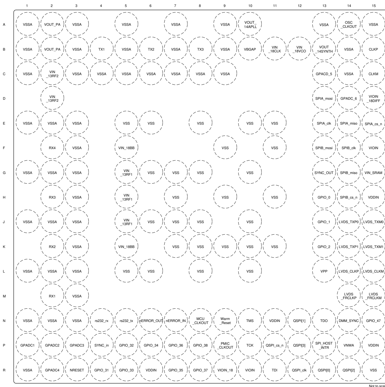
Figure 6-1. Pin Diagram
