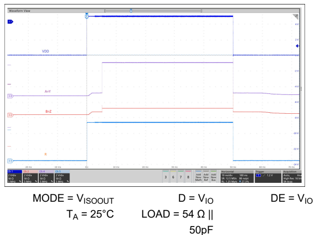
Figure 8-32. Glitch-free Power up/down- Profibus Mode
