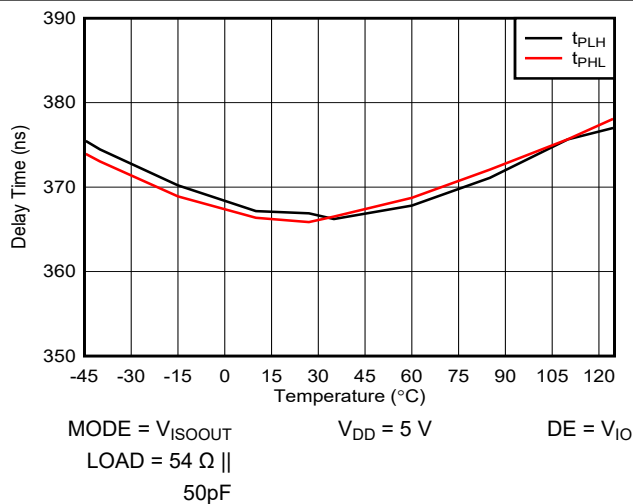
Figure 8-13. ISOW1412 Driver Propagation Delay vs. Temperature - Profibus Mode
