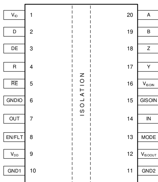
Figure 7-1. ISOW14x2 20-pin DFM Top View
