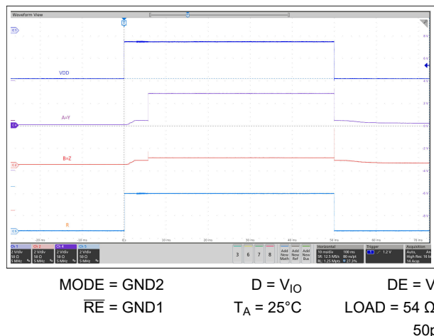
Figure 8-31. Glitch-free Power up/down- RS485 Mode
