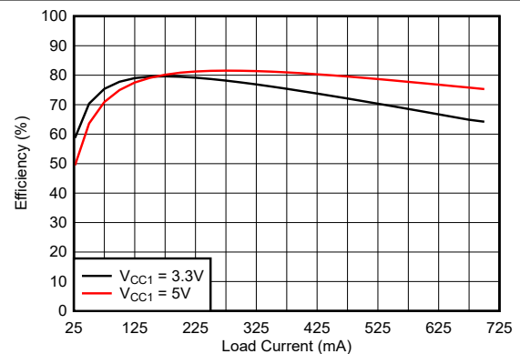
Figure 5-14. ISO774xTB-Q1 Efficiency vs. Load Current
